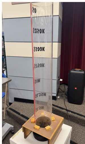
Wind Tunnel
